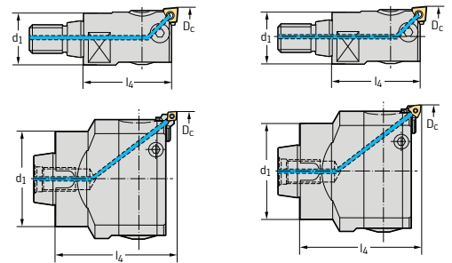
Complete tool
