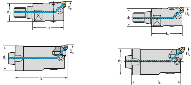
Complete tool
